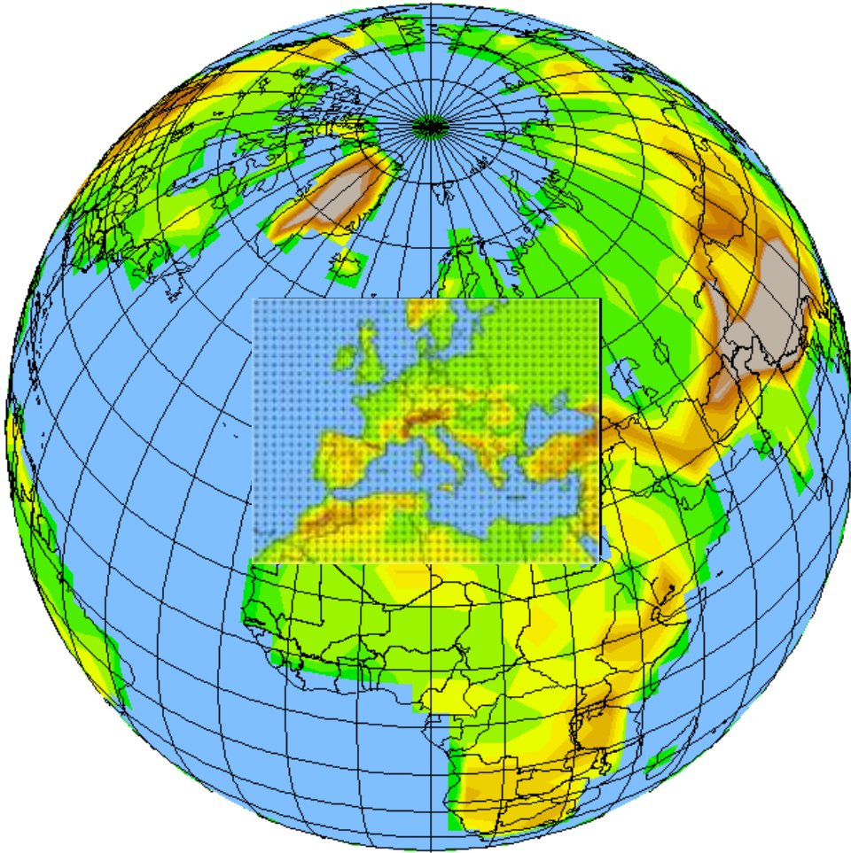
Fig. 3 Nested regional climate model.
